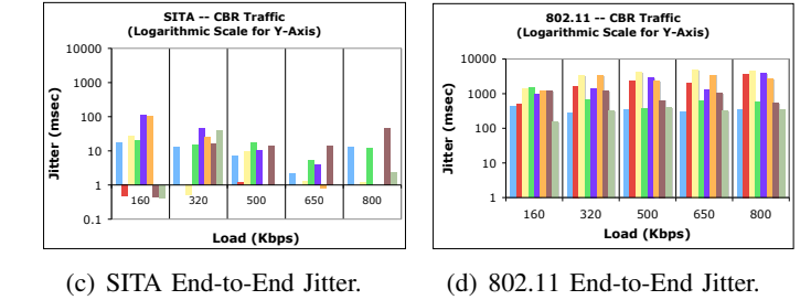
Fig. 6. Experiment 1: 8 by 8 Manhattan grid; 8 flows generating CBR traffic. At high loads, IEEE 802.11 becomes extremely unfair, resulting in many flows experiencing very high end-to-end delay and jitter. SITA delivers the data on all the flows at very low end-to-end delay and jitter.
