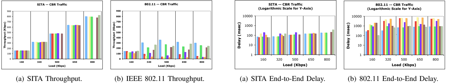
Fig. 4. Experiment 1: 8 by 8 Manhattan grid; 8 flows generating CBR traffic. At high loads, IEEE 802.11 becomes extremely unfair, resulting in high variance in realized throughputs among flows. SITA, on the other hand, delivers fair throughput to as many flows as possible.
