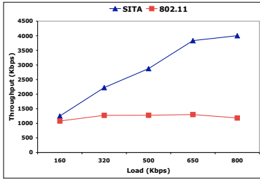
Fig. 5. Experiment 1: 8 by 8 Manhattan grid; 8 flows generating CBR traffic. SITA offers several times increase in the overall network throughput for moderate to high loads.
