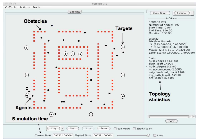
Fig. 5. VizTools snapshot view of Manhattan model execution delivered. Two types of nodes are defined: (1) regular nodes, and (2) message ferries. Regular nodes can be static or mobile; message ferries are intended to visit regular nodes according to some routing specification with the purpose of getting and delivering data messages from and to them. This mobility scenario has a wide variety of applications, and research for specific domains involves the design and analysis of route layouts for the message ferries.
