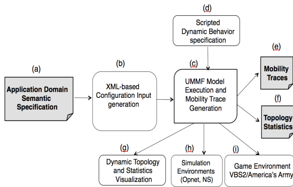
Fig. 4. High-Level UMMF Flow Diagram.
