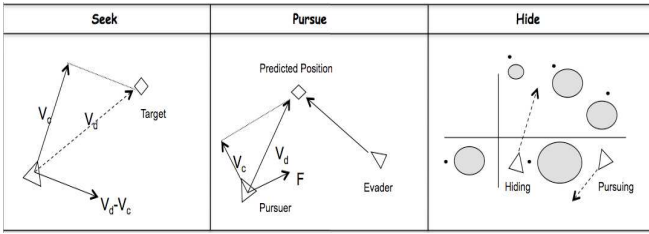
Fig. 2. Individual Steering Forces
