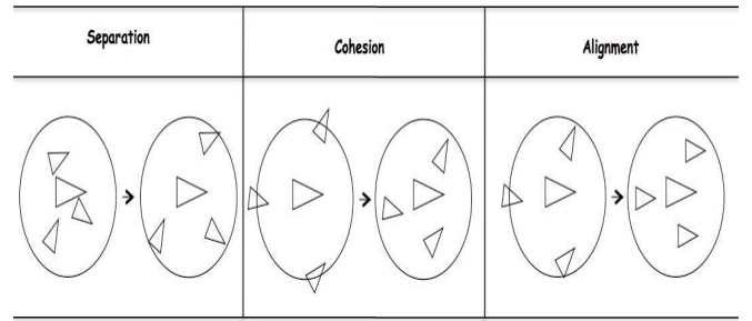
Fig. 3. Combination of Individual Steering Forces to achieve flocking
