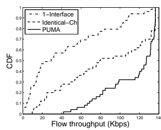
Figure 3: CDF of flow throughput.
