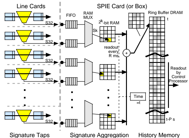
Figure 8: A sample SPIE DGA hardware implementation for high-speed routers.
