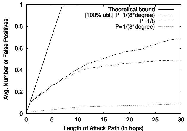
Figure 9: The number of false positives in a SPIE-generated attack graph as a function of the length of the attack path, for p = 1/8 . The theoretical bound is plotted against three simulation results, two with false-positive rates conditioned on router degree, one without. For the two degree-dependent runs, one considered actual link utilization, while the other assumed full utilization. Each simulation represents the average of 5000 runs using actual topology and utilization data from a national tier-one ISP.
