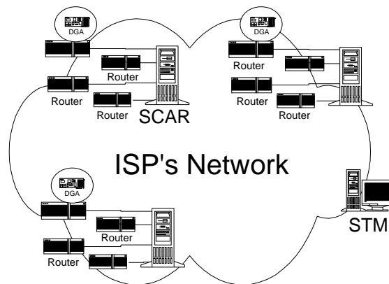
Figure 5: The SPIE network infrastructure, consisting of Data Generation Agents (DGAs), SPIE Collection and Reduction Agents (SCARs), and a SPIE Traceback Manager (STM).
